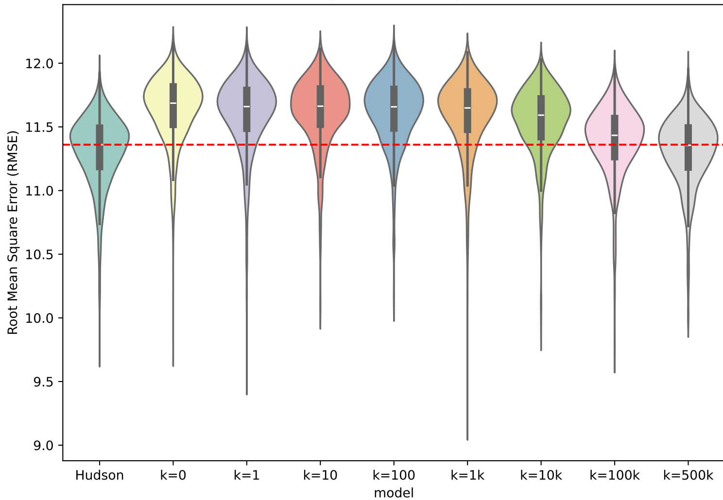
TSCompare RMSE Comparison
