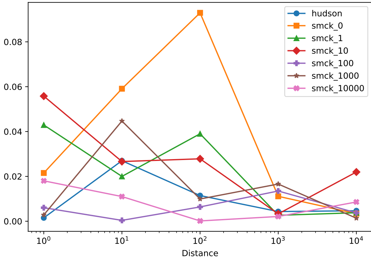
Error in Covariance of TMRCA at distance d
