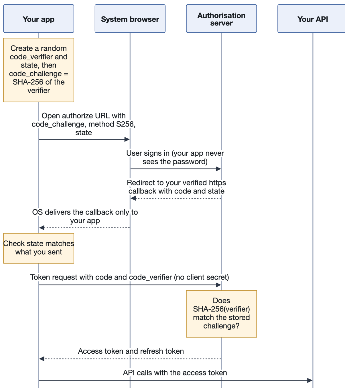
Figure 2: Sign-in with the authorisation code flow and PKCE, through the system browser
