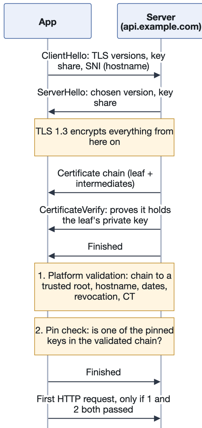
Figure 8: A TLS 1.3 handshake, and where the pin check sits
