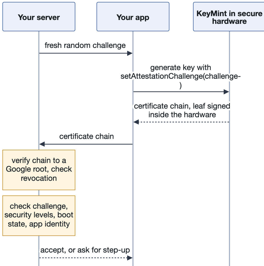
Figure 6: Key attestation: the server's challenge comes back inside a certificate chain signed by the hardware
