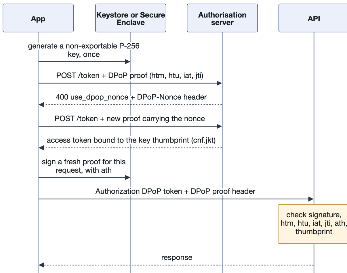
Figure 15: DPoP: every request carries a fresh proof signed by a device-bound key
