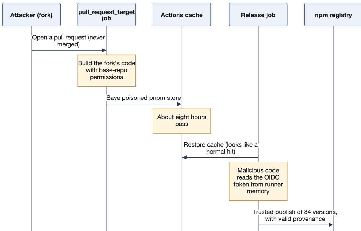
Figure 19: The TanStack compromise: a poisoned cache crosses from an untrusted job into the release job
