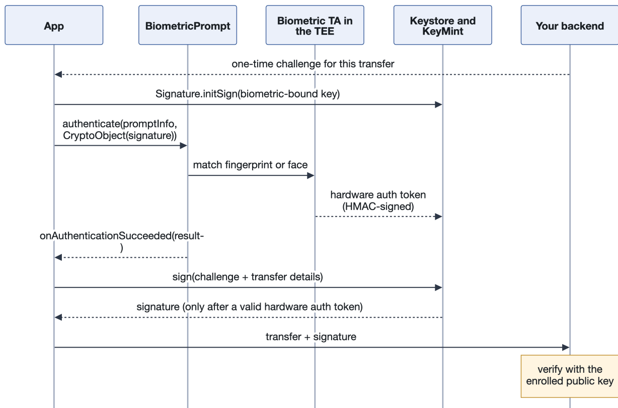
Figure 13: A biometric prompt that unlocks a key, rather than flipping a boolean
