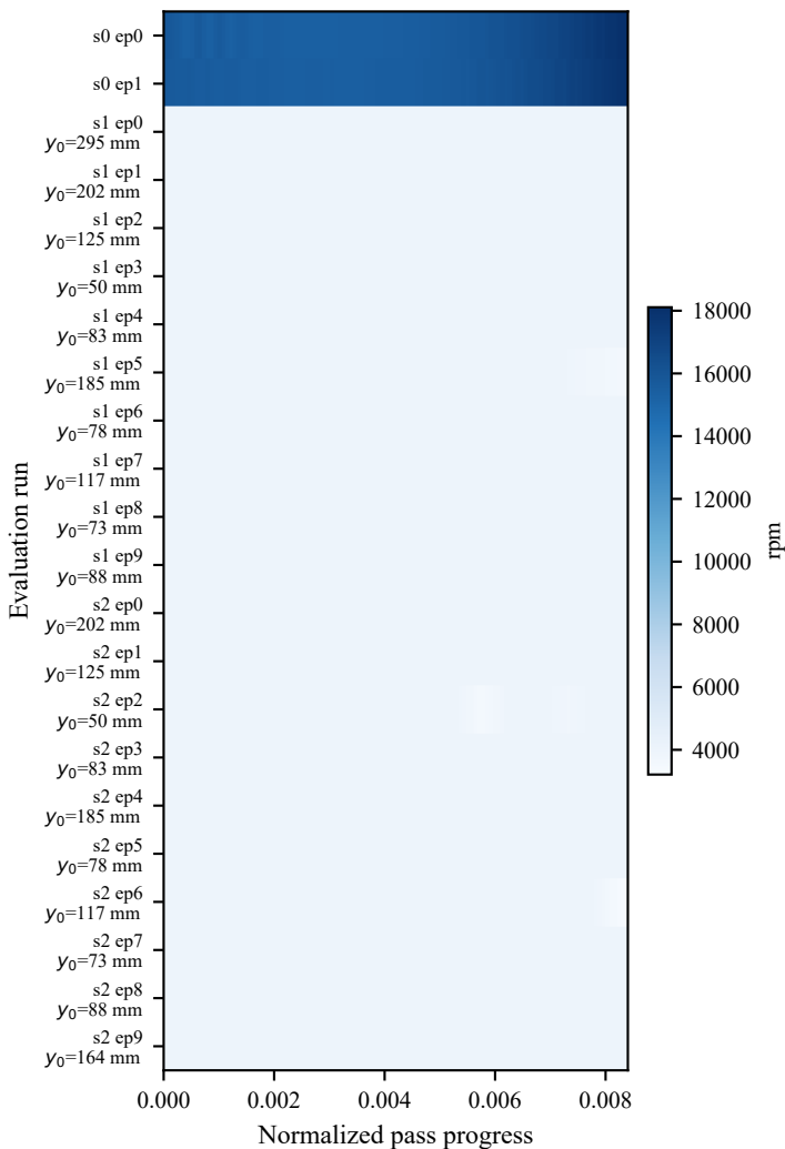
Spindle speed (rpm)
