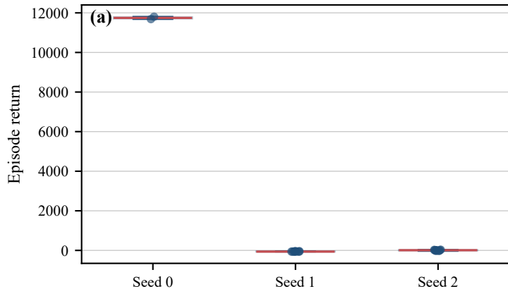
Return distribution
