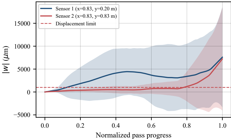
Per-sensor vibration ensemble (mean \pm 3\sigma , n=22)
