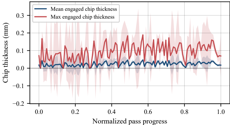
Cutting-process ensemble (mean \pm 3\sigma , n=2)
