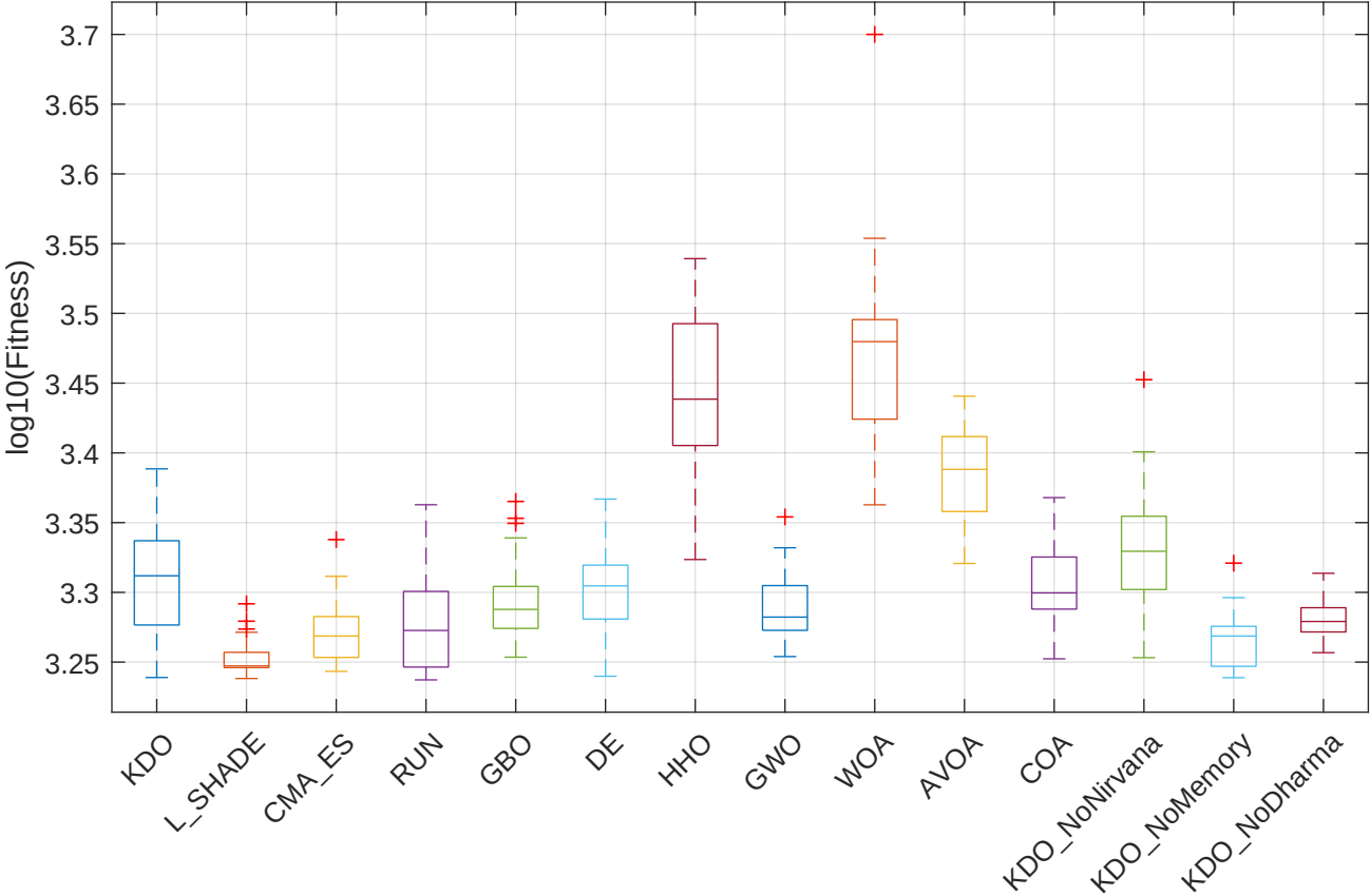
CEC2017 F17 (Numerical) - Boxplot
