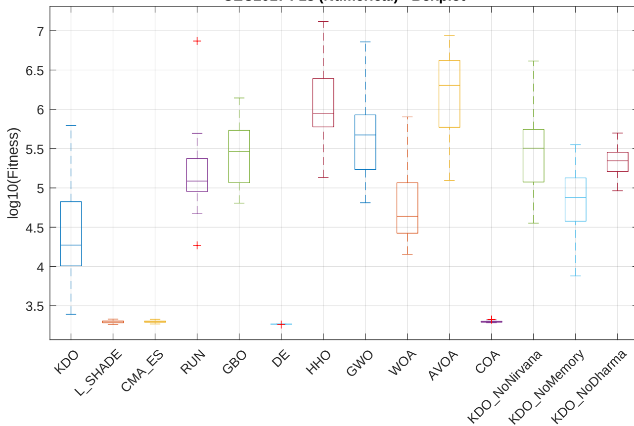
CEC2017 F18 (Numerical) - Boxplot
