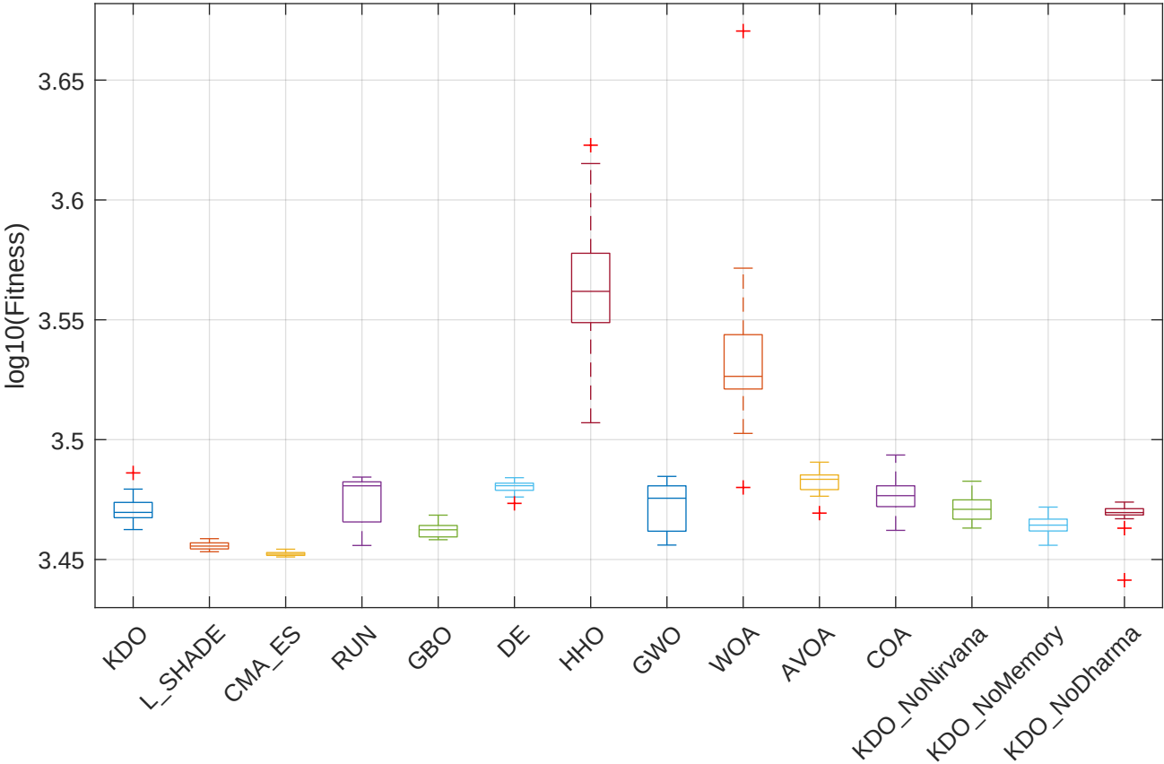
CEC2017 F24 (Numerical) - Boxplot
