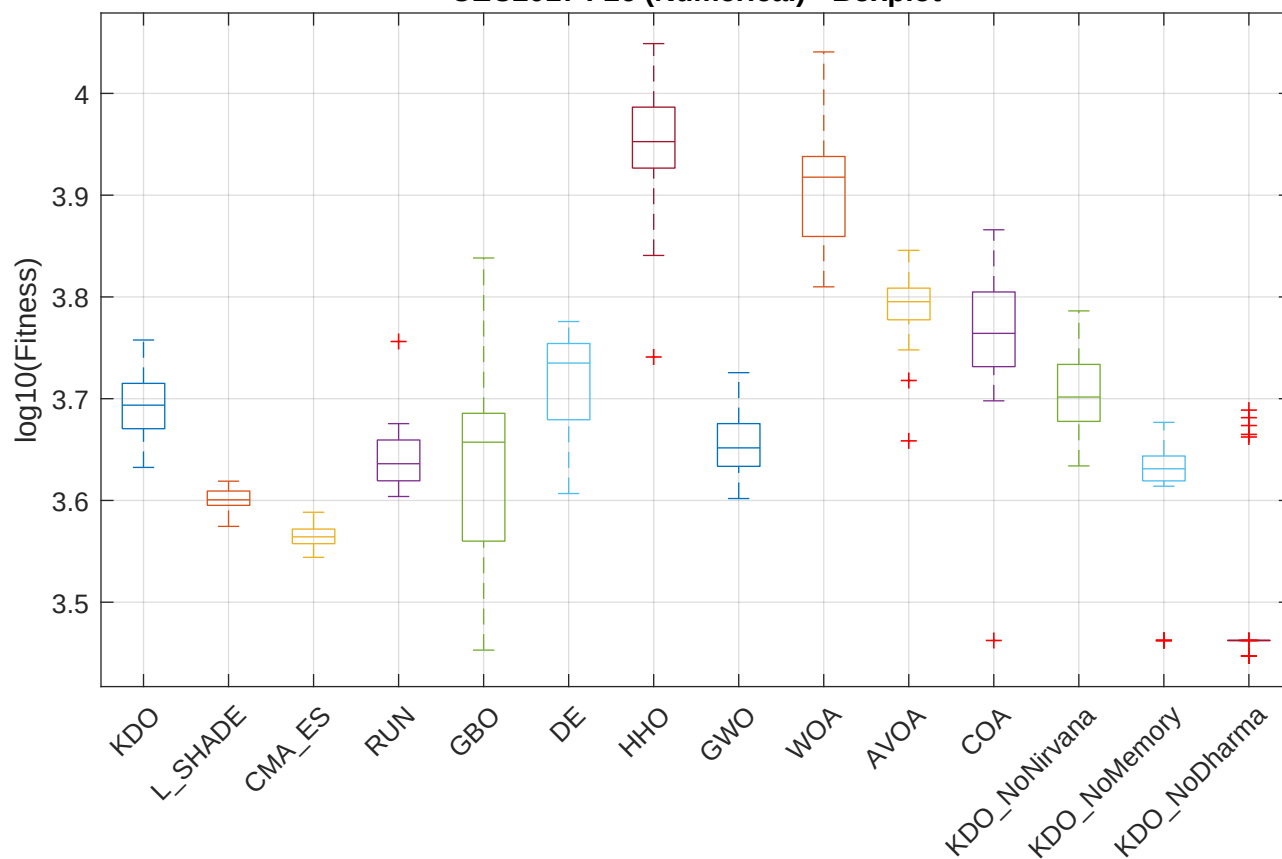
CEC2017 F26 (Numerical) - Boxplot
