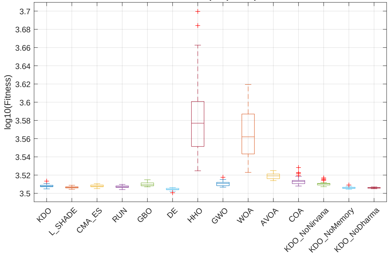
CEC2017 F27 (Full) - Boxplot
