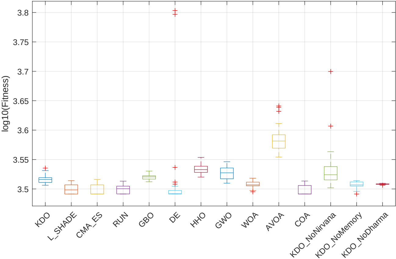
CEC2017 F28 (Numerical) - Boxplot
