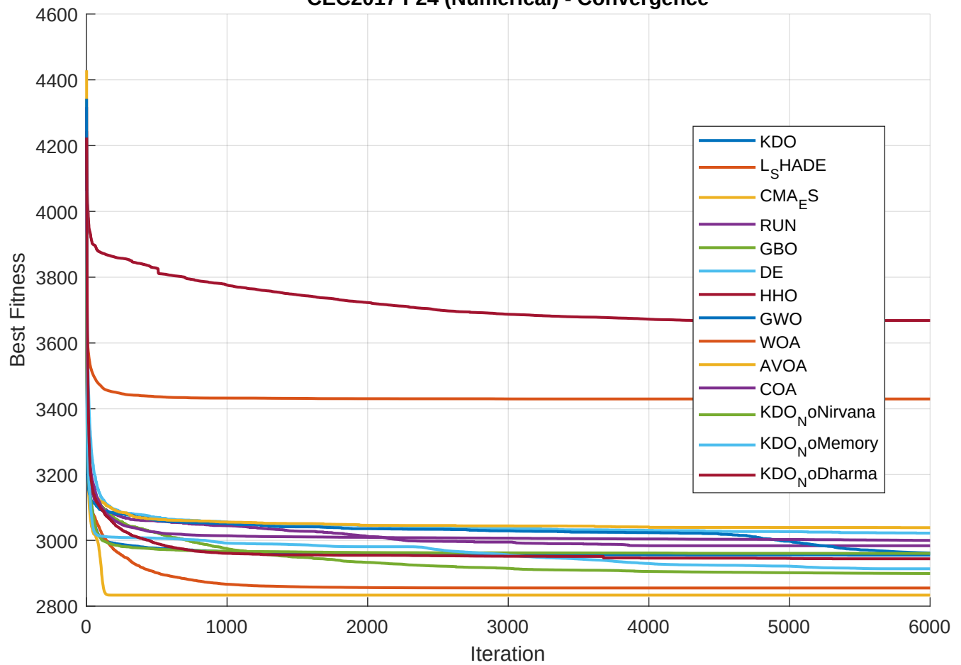
CEC2017 F24 (Numerical) - Convergence
