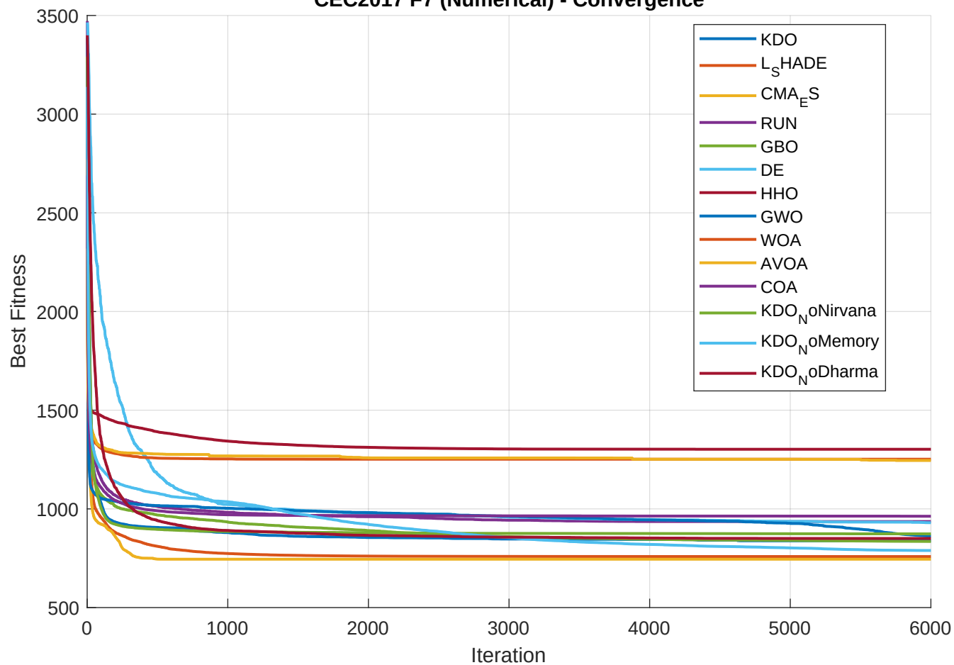
CEC2017 F7 (Numerical) - Convergence
