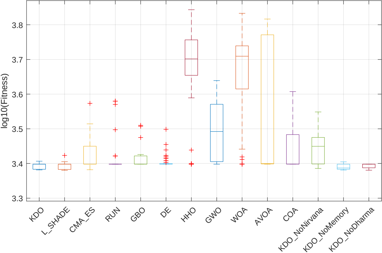
CEC2022 F10 (Numerical) - Boxplot
