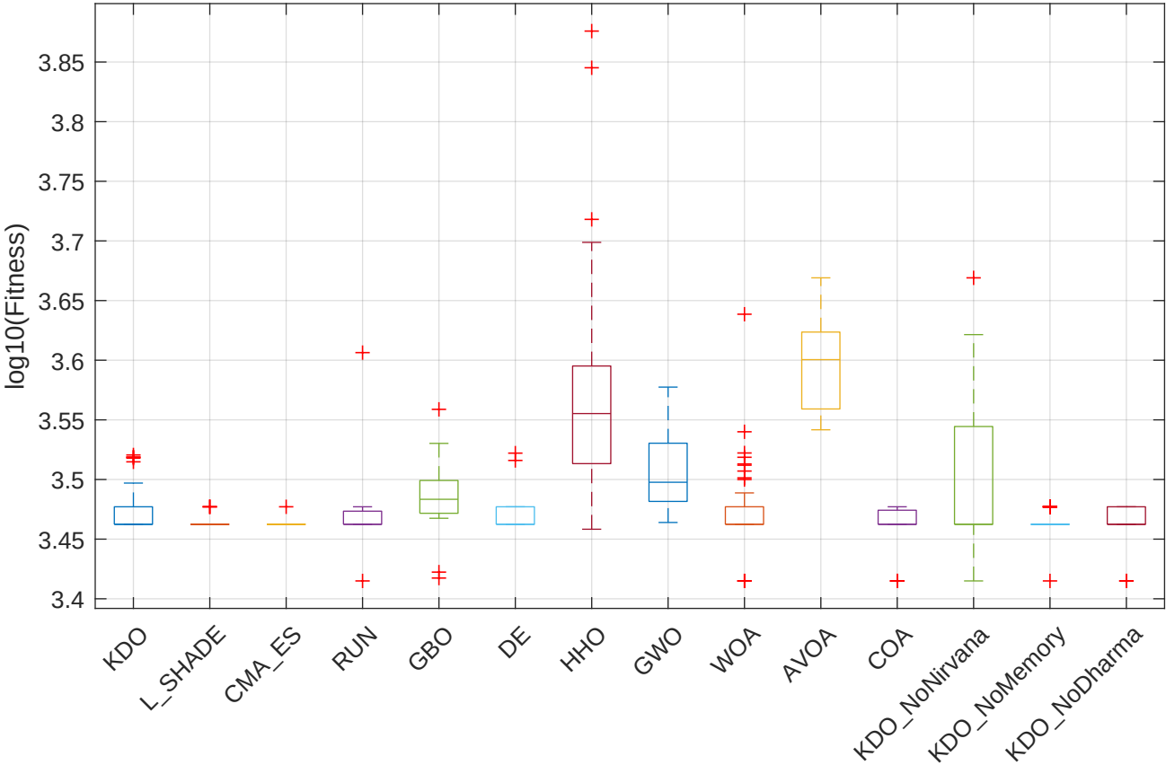
CEC2022 F11 (Numerical) - Boxplot
