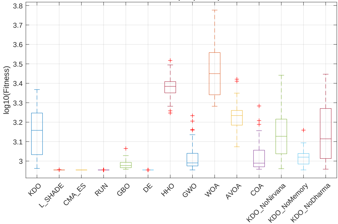
CEC2022 F5 (Full) - Boxplot
