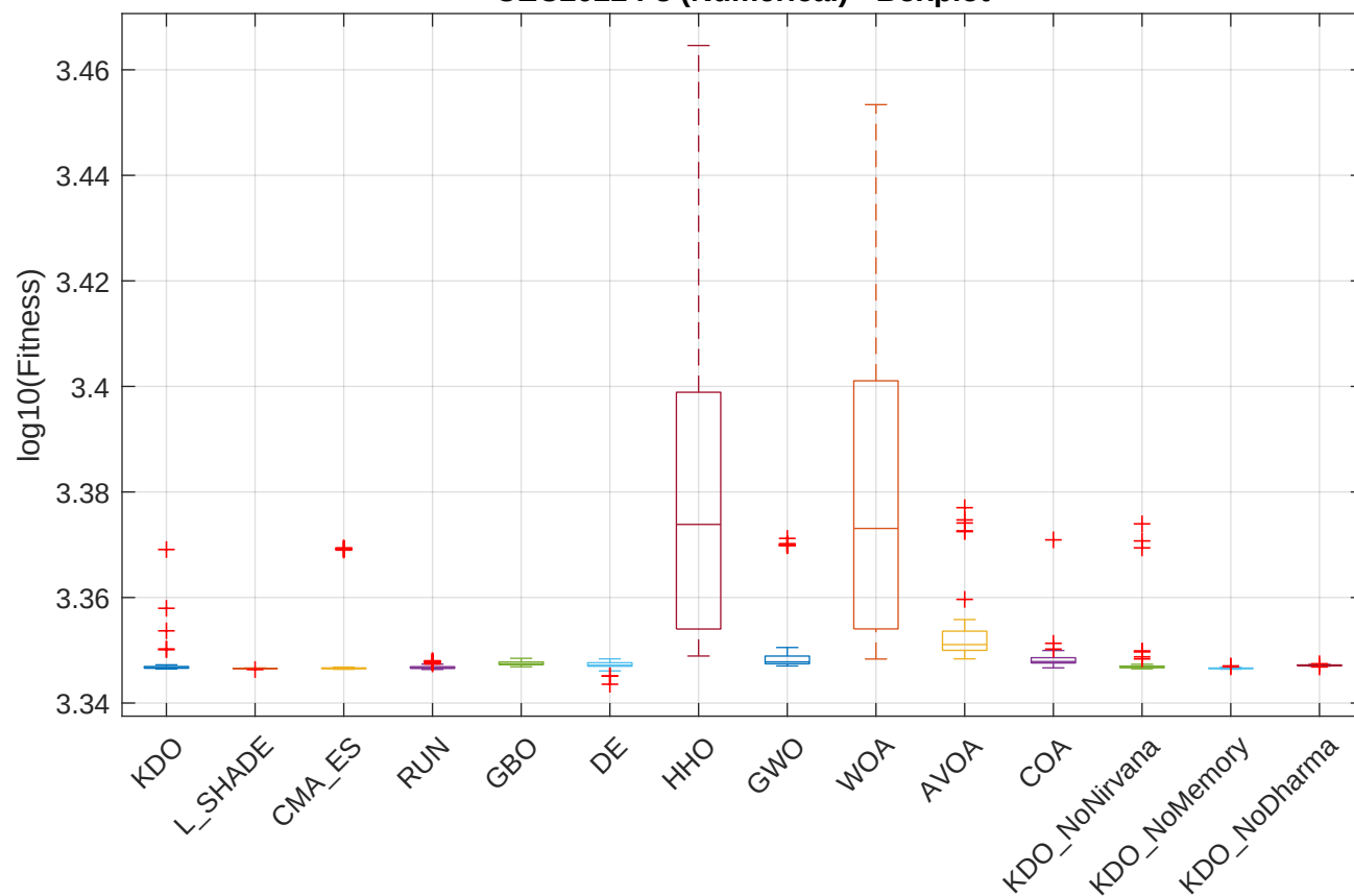
CEC2022 F8 (Numerical) - Boxplot
