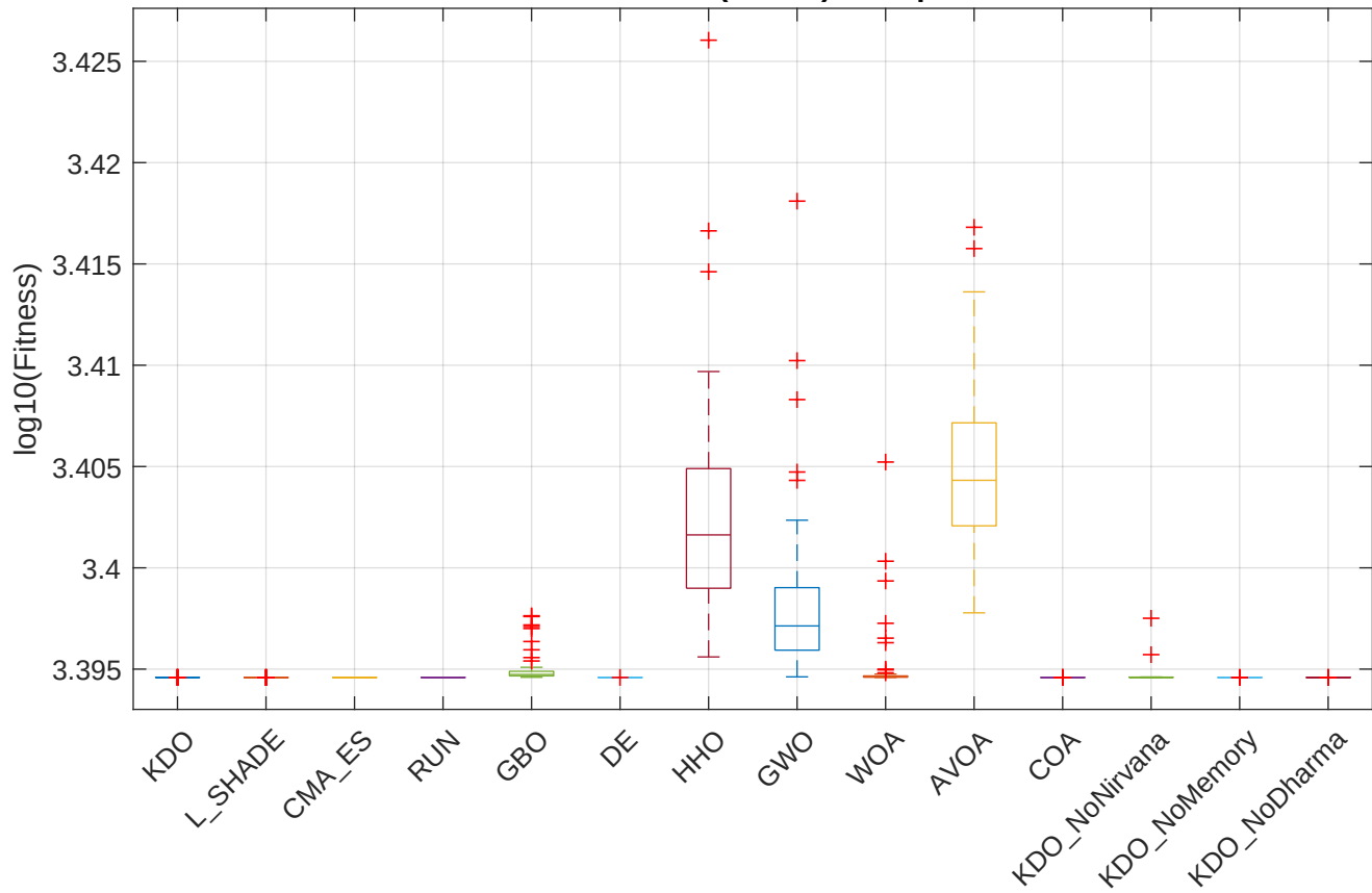
CEC2022 F9 (Partial) - Boxplot
