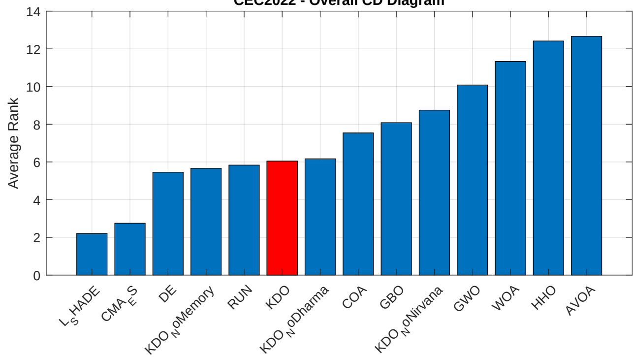
CEC2022 - Overall CD Diagram
