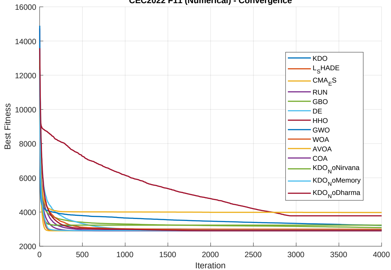
CEC2022 F11 (Numerical) - Convergence
