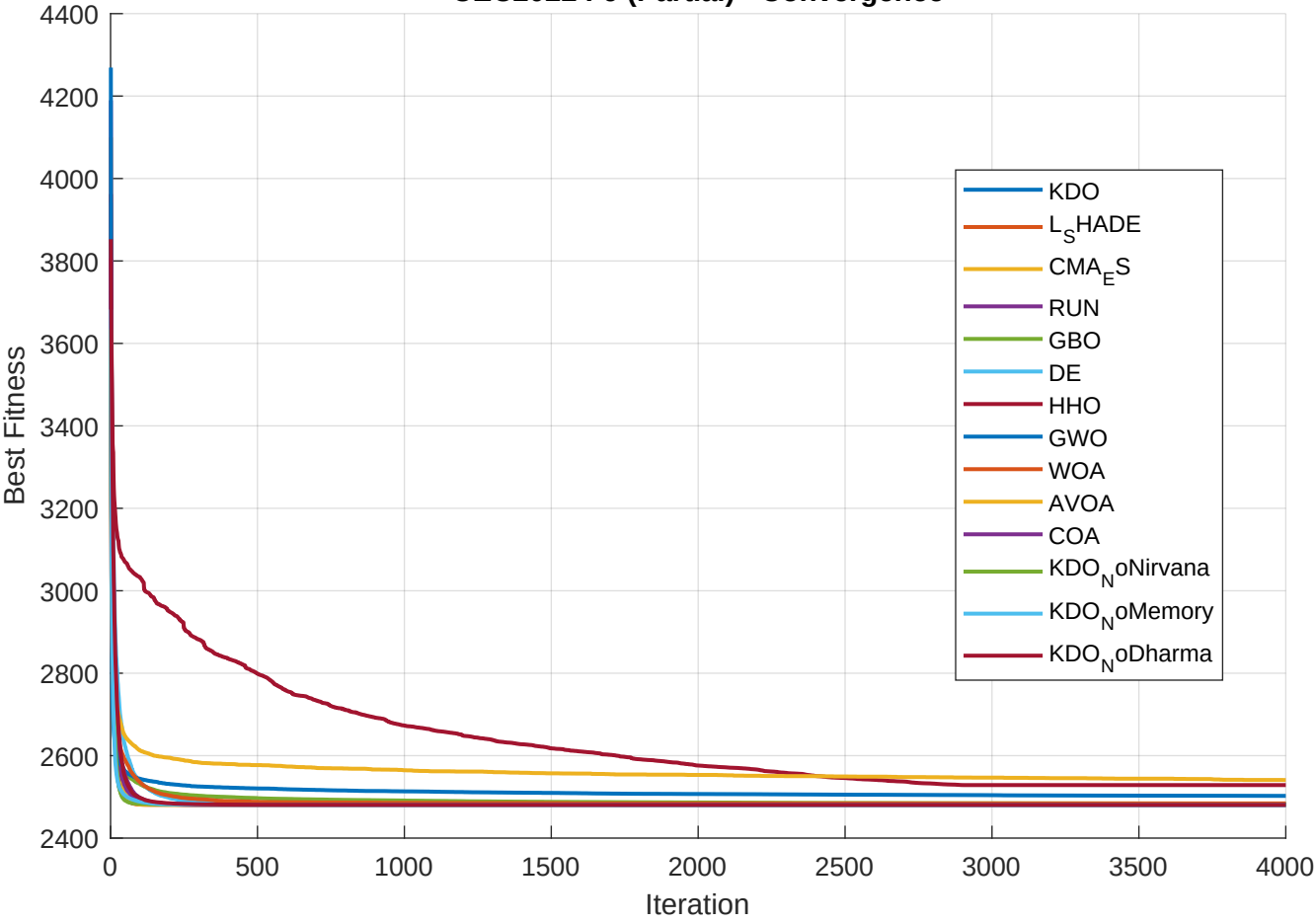
CEC2022 F9 (Partial) - Convergence
