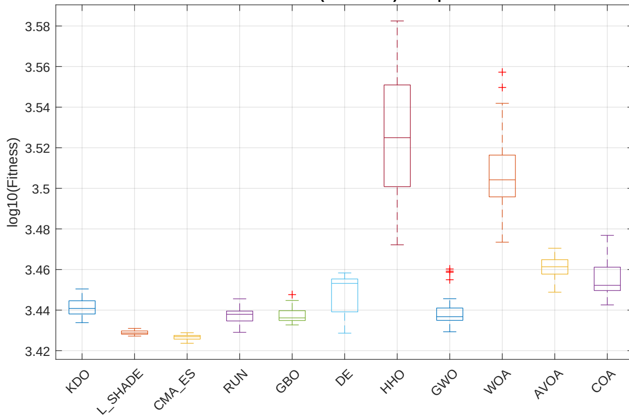
CEC2017 F23 (Numerical) - Boxplot
