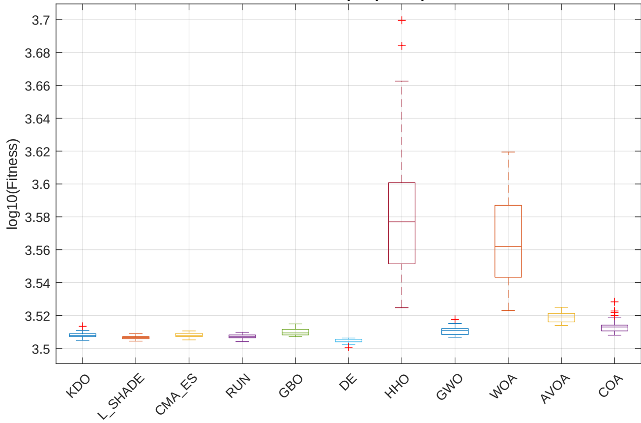
CEC2017 F27 (Full) - Boxplot
