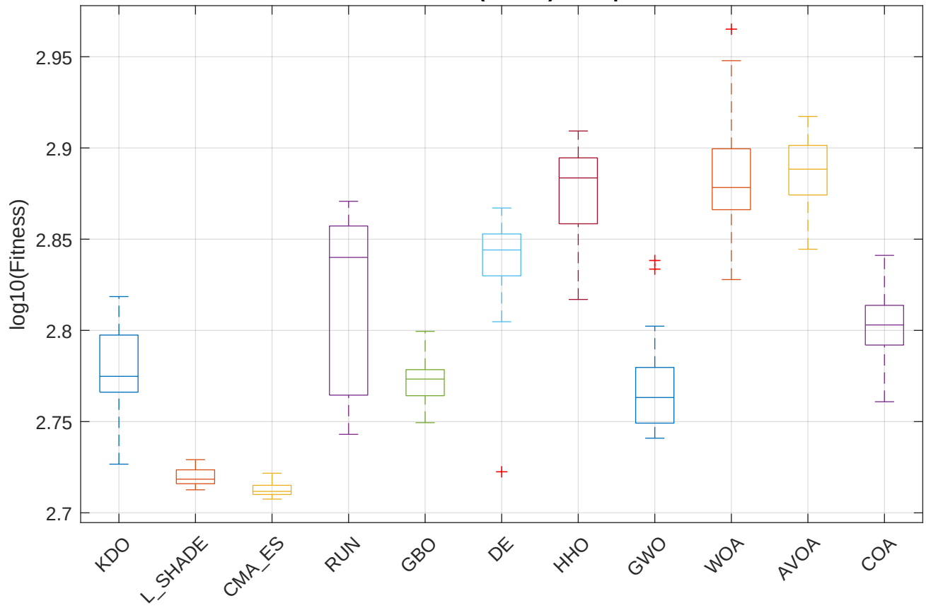
CEC2017 F5 (Partial) - Boxplot
