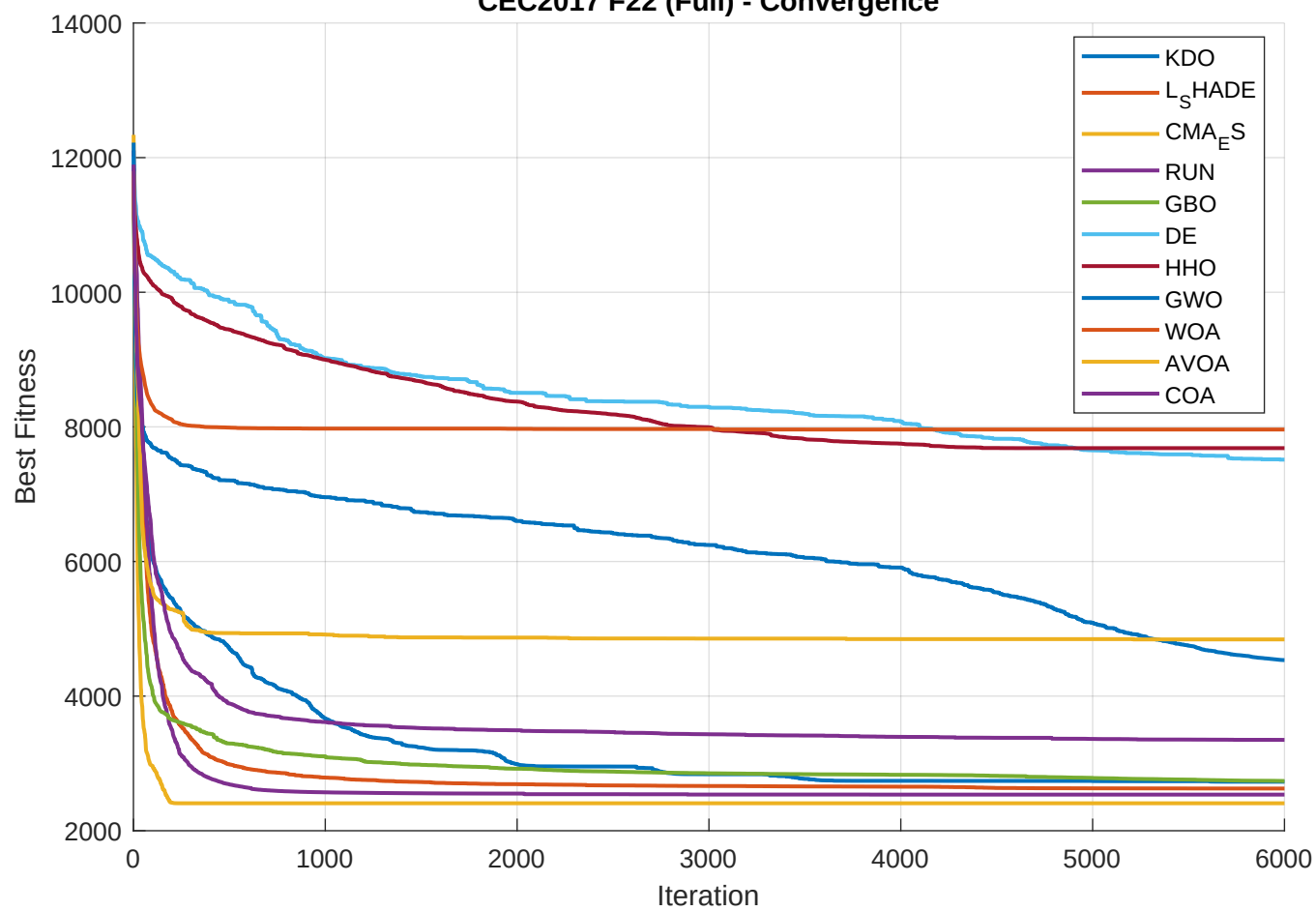
CEC2017 F22 (Full) - Convergence
