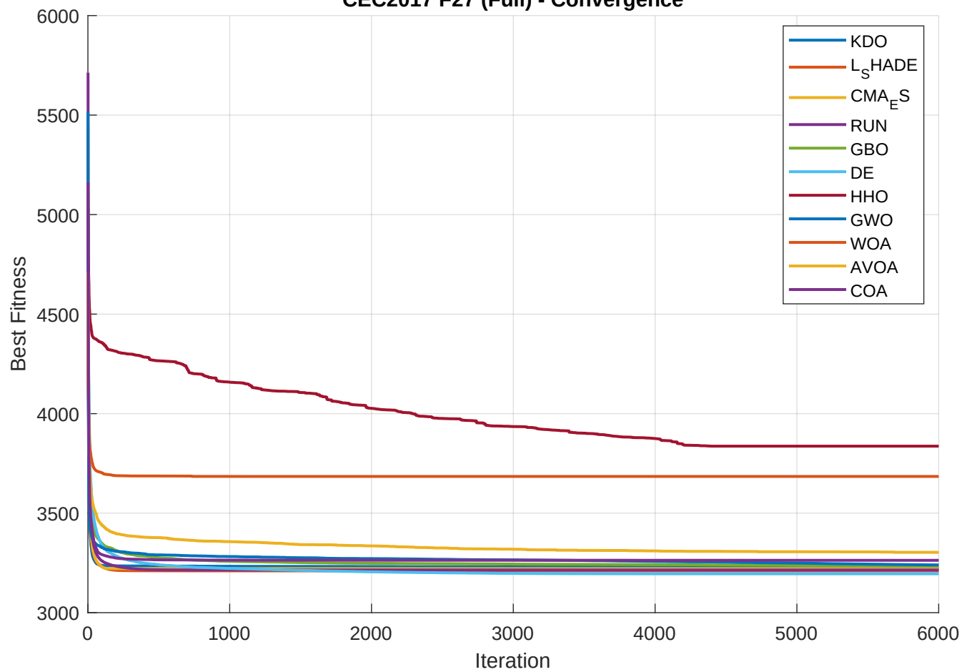
CEC2017 F27 (Full) - Convergence
