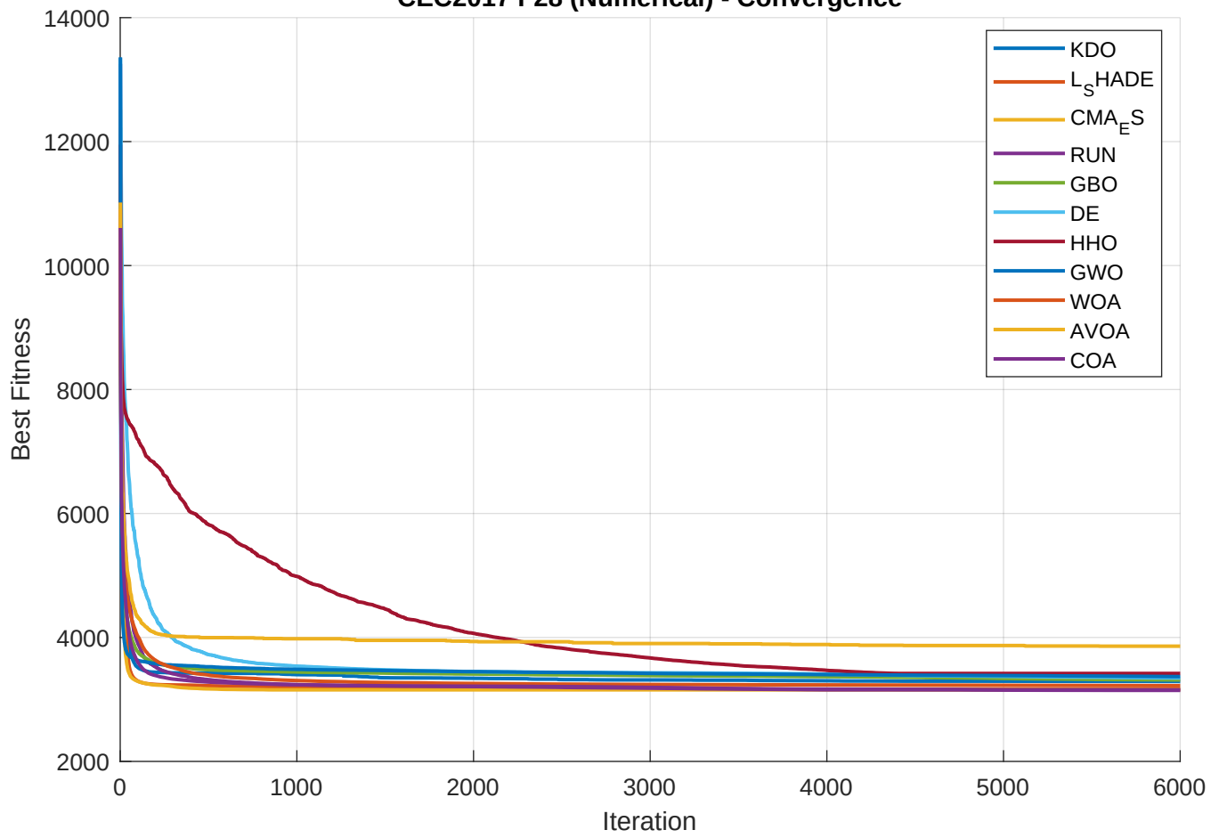
CEC2017 F28 (Numerical) - Convergence
