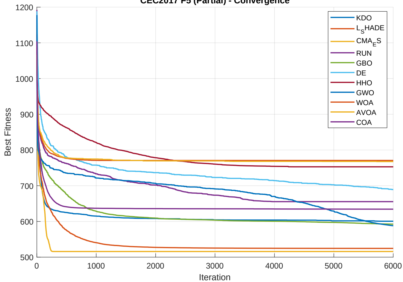
CEC2017 F5 (Partial) - Convergence
