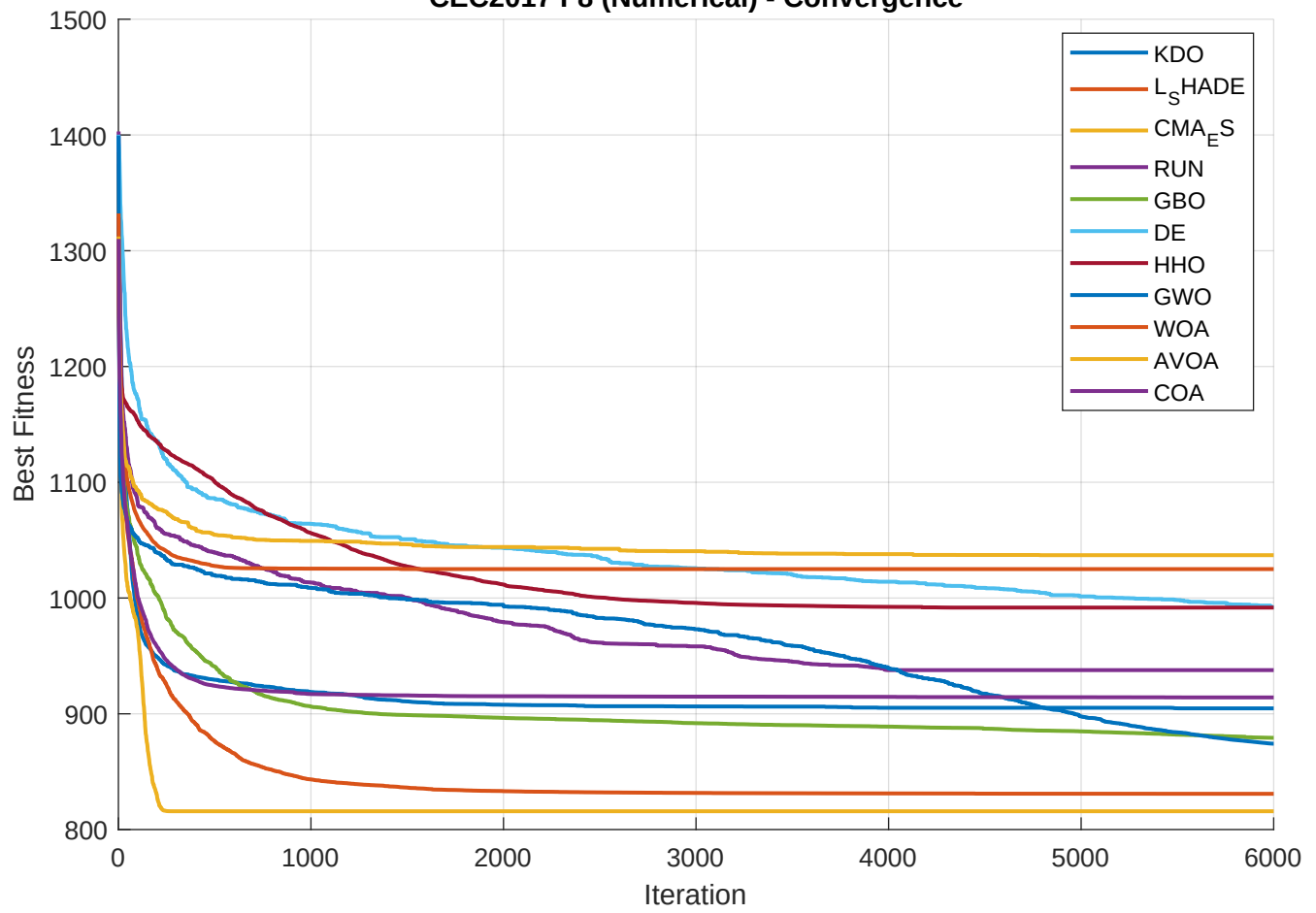
CEC2017 F8 (Numerical) - Convergence
