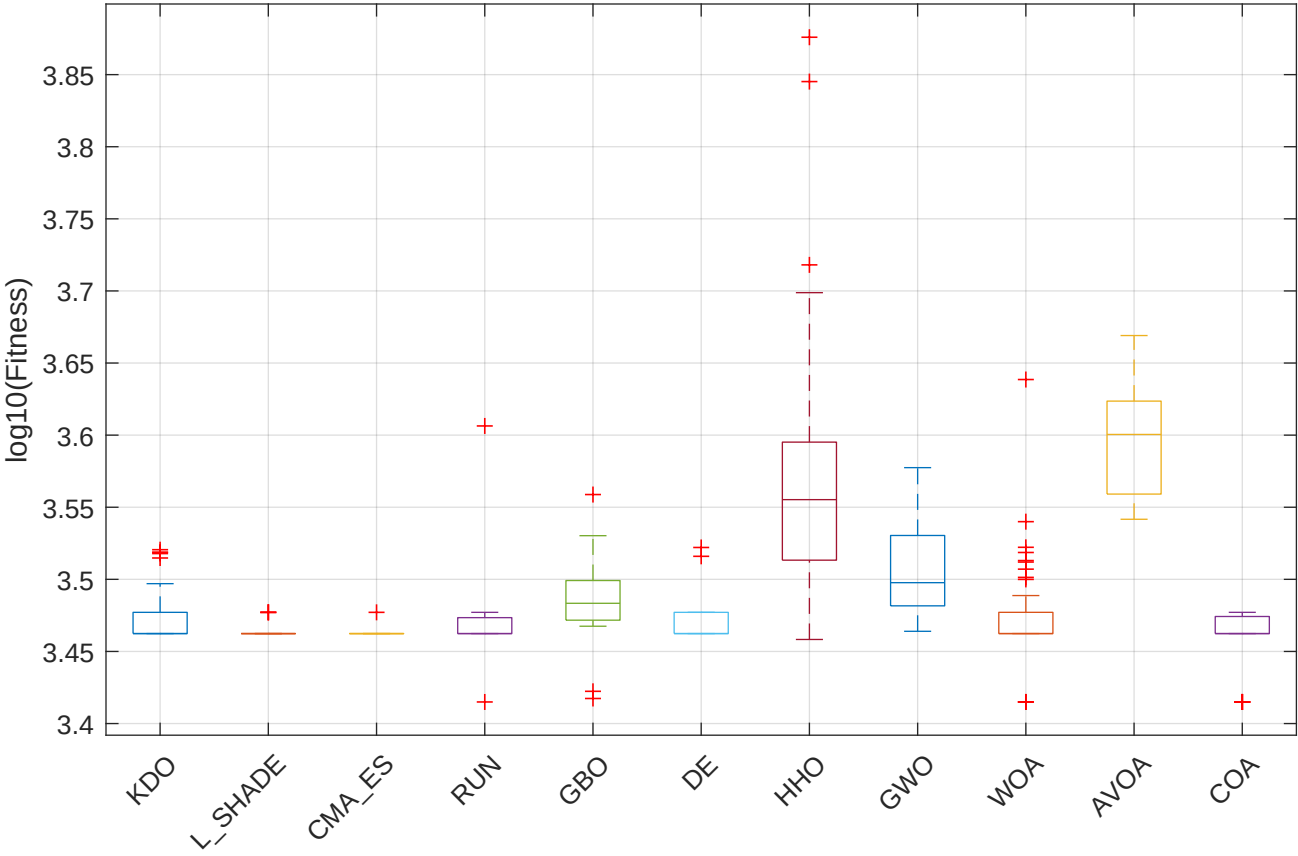
CEC2022 F11 (Numerical) - Boxplot
