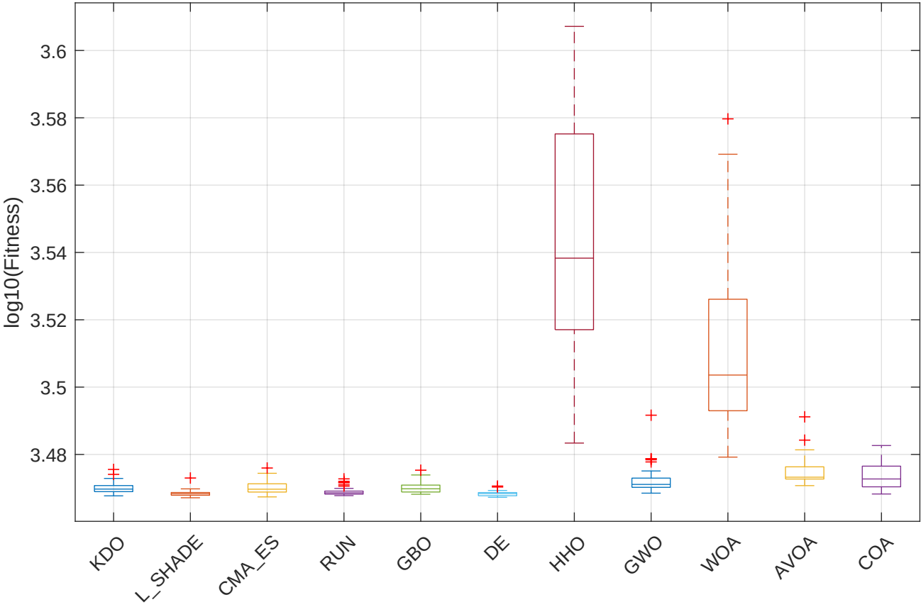
CEC2022 F12 (Numerical) - Boxplot
