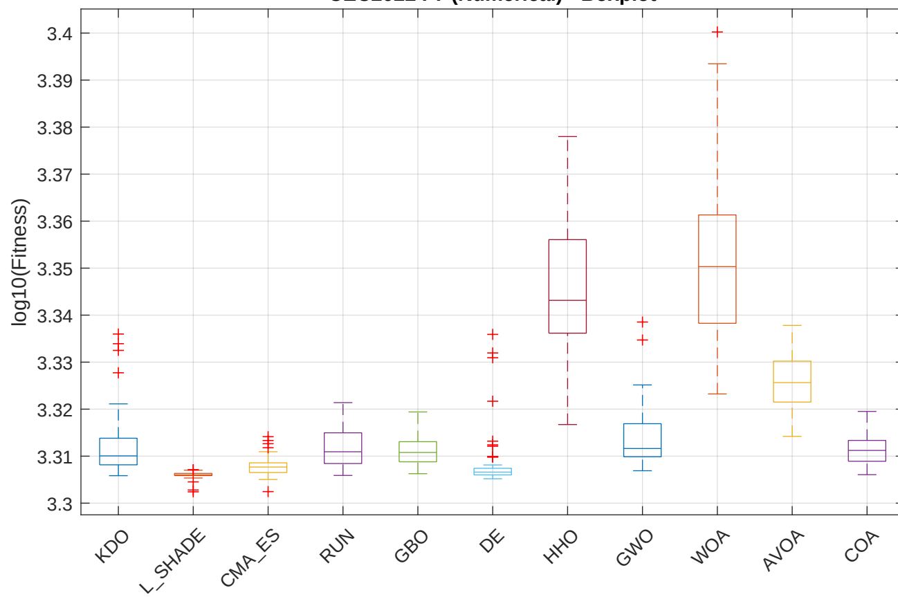
CEC2022 F7 (Numerical) - Boxplot
