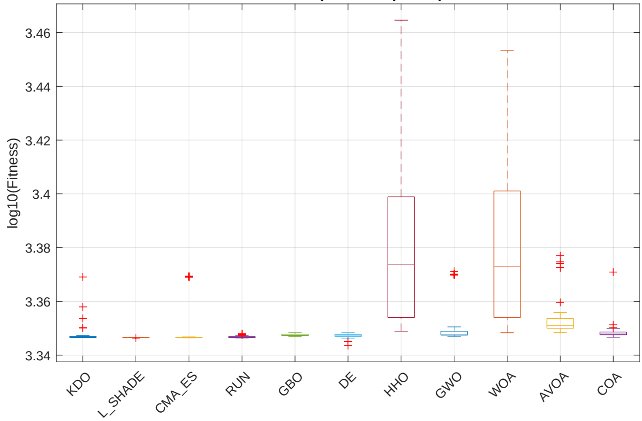
CEC2022 F8 (Numerical) - Boxplot
