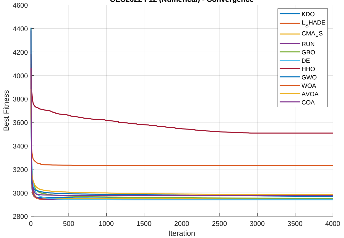
CEC2022 F12 (Numerical) - Convergence
