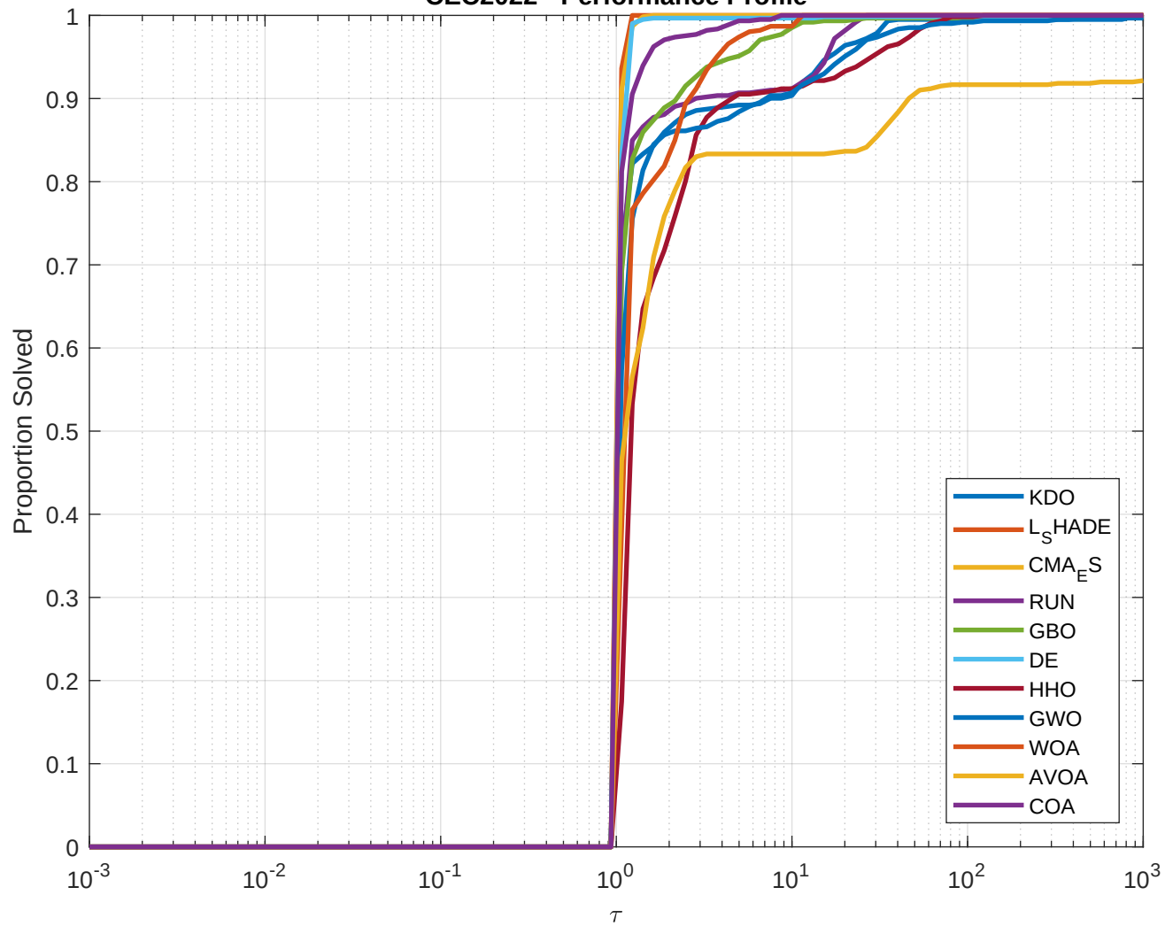
CEC2022 - Performance Profile
