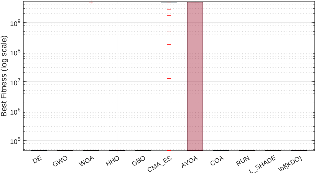
Box Plot - E2: RF CMOS Cascode LNA 2.4GHz (12D) - HARD with Noise
