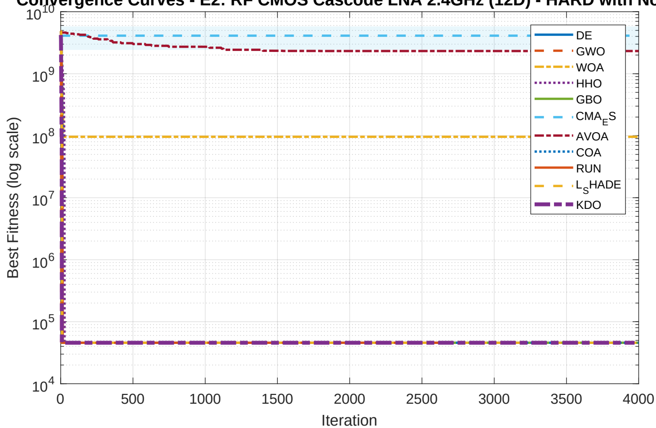
Convergence Curves - E2: RF CMOS Cascode LNA 2.4GHz (12D) - HARD with Noise
