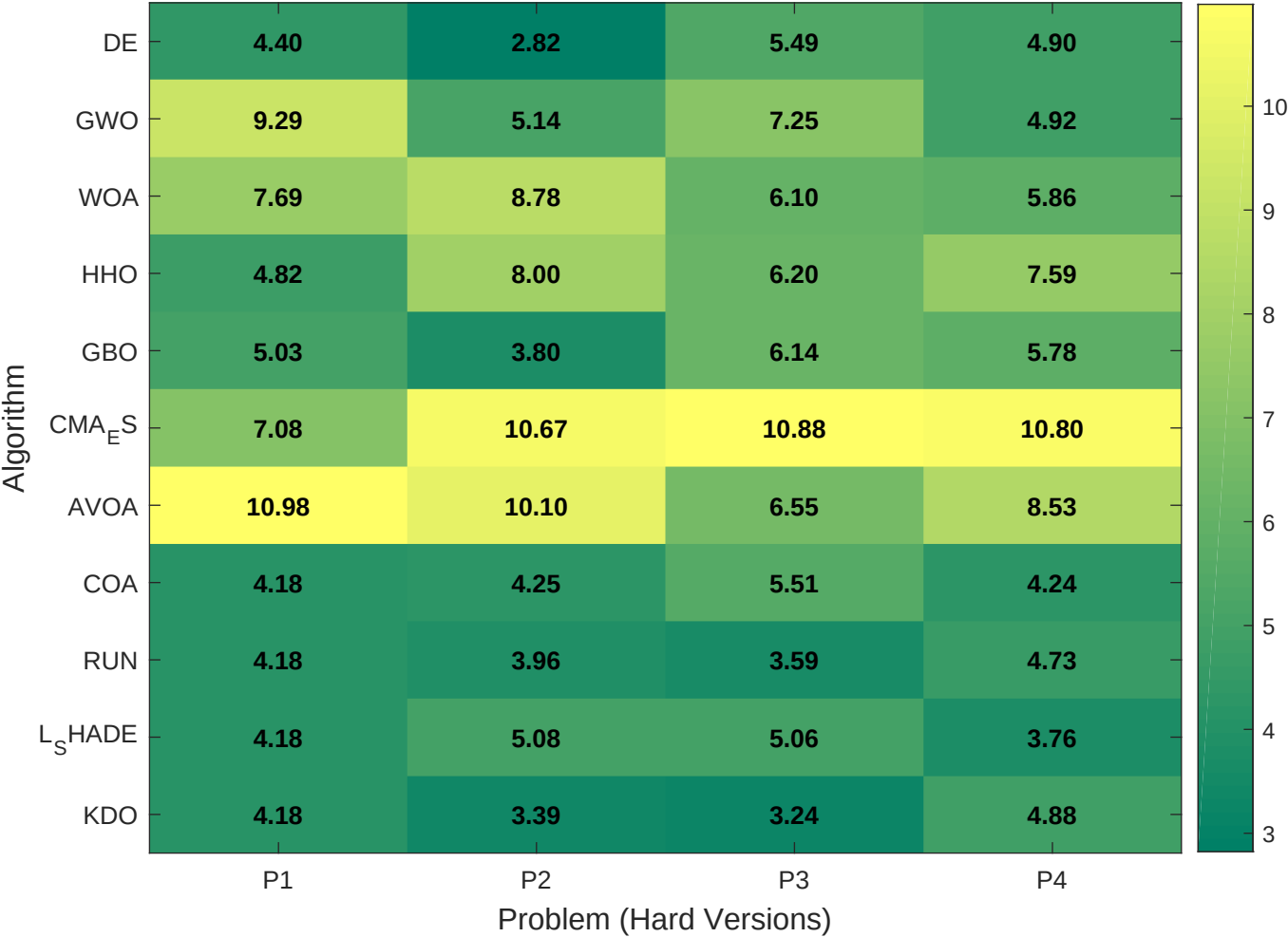
Friedman Rank Heatmap (lower is better)
