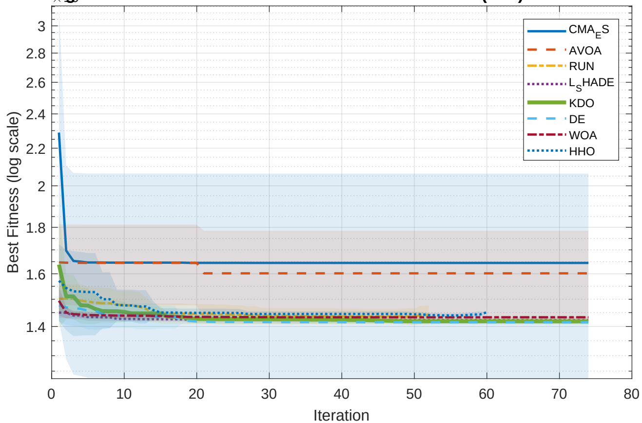
Convergence Curves - E2: RF CMOS Cascode LNA 2.4GHz (12D) - HARD with Noise
