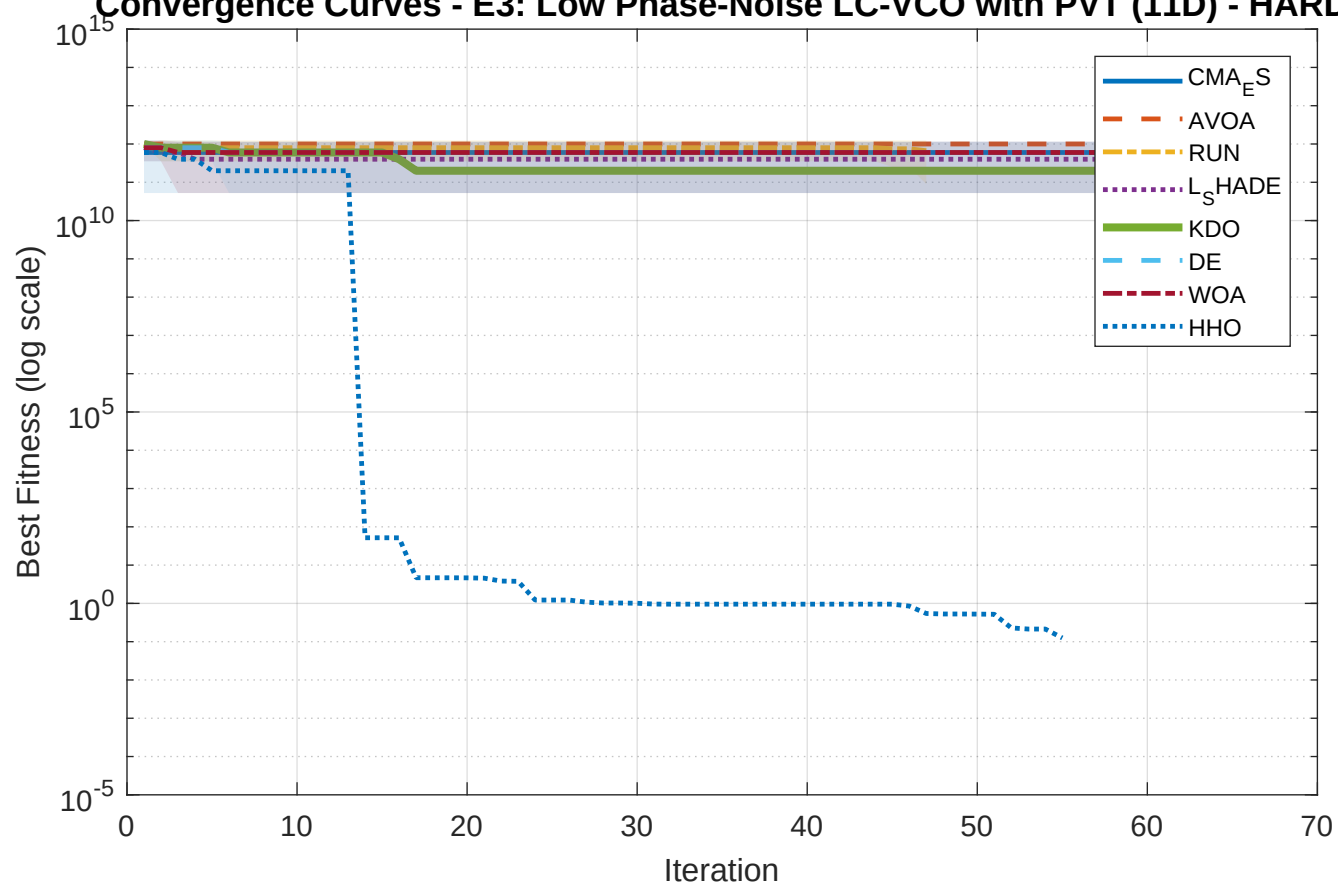
15 Convergence Curves - E3: Low Phase-Noise LC-VCO with PVT (11D) - HARD
