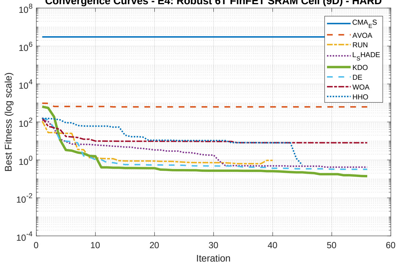
Convergence Curves - E4: Robust 6T FinFET SRAM Cell (9D) - HARD
