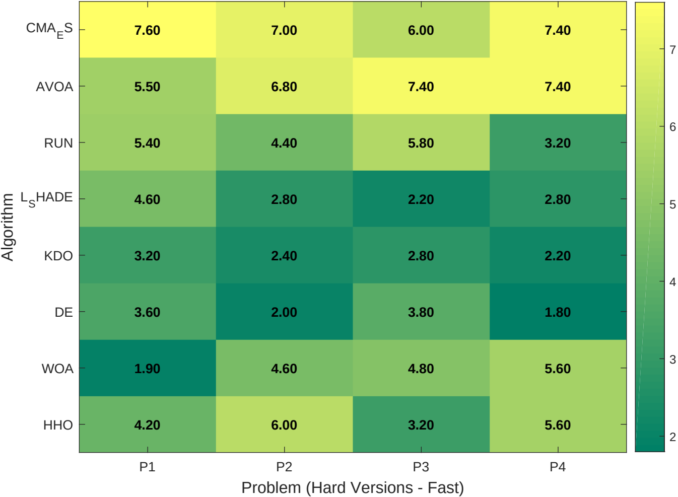
Friedman Rank Heatmap (lower is better) - Fast
