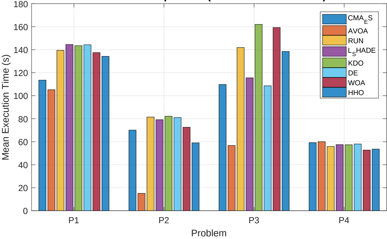
Runtime Comparison (Hard Problems - Fast)
