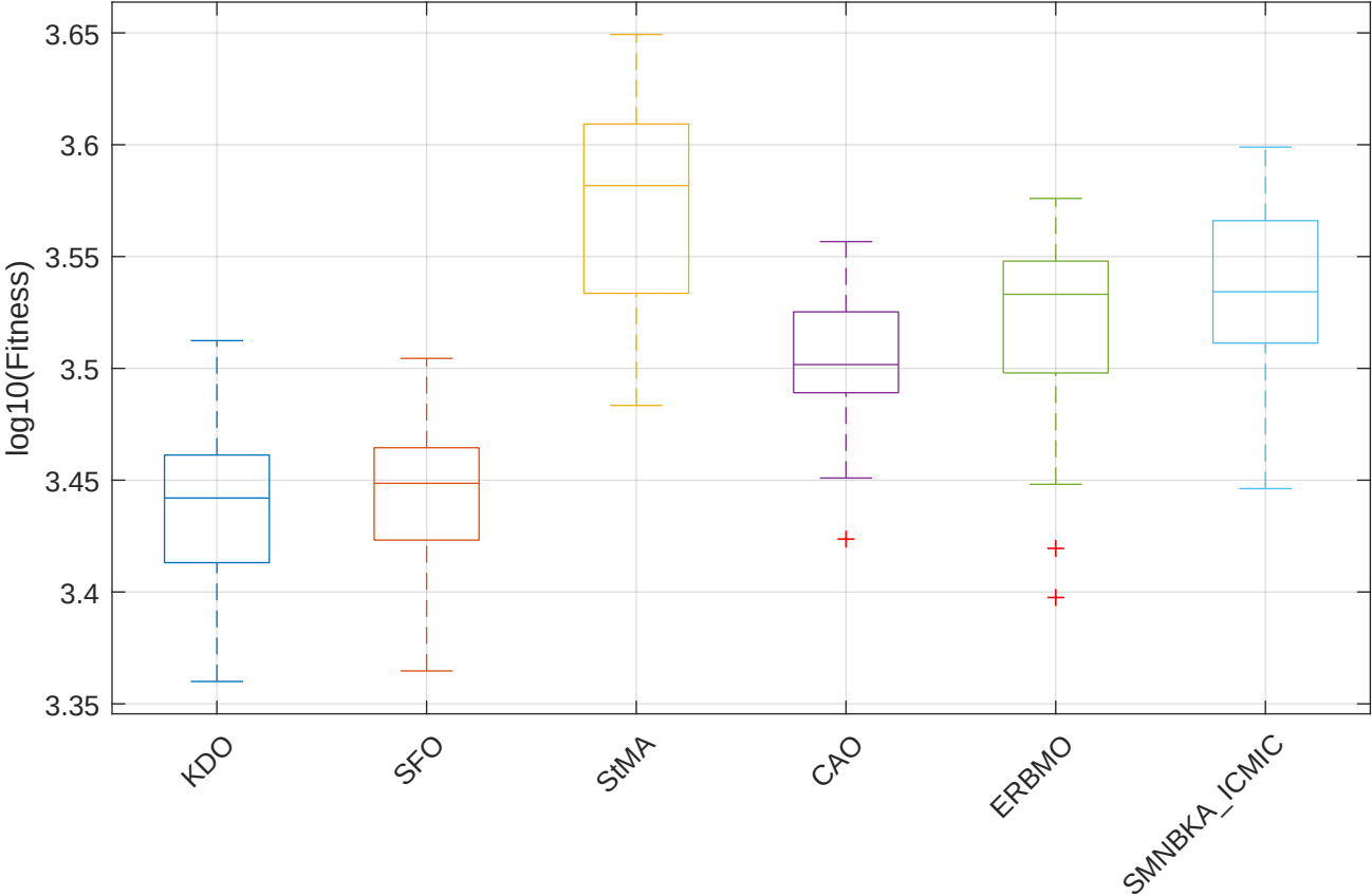
CEC2017 F20 (Numerical) - Boxplot
