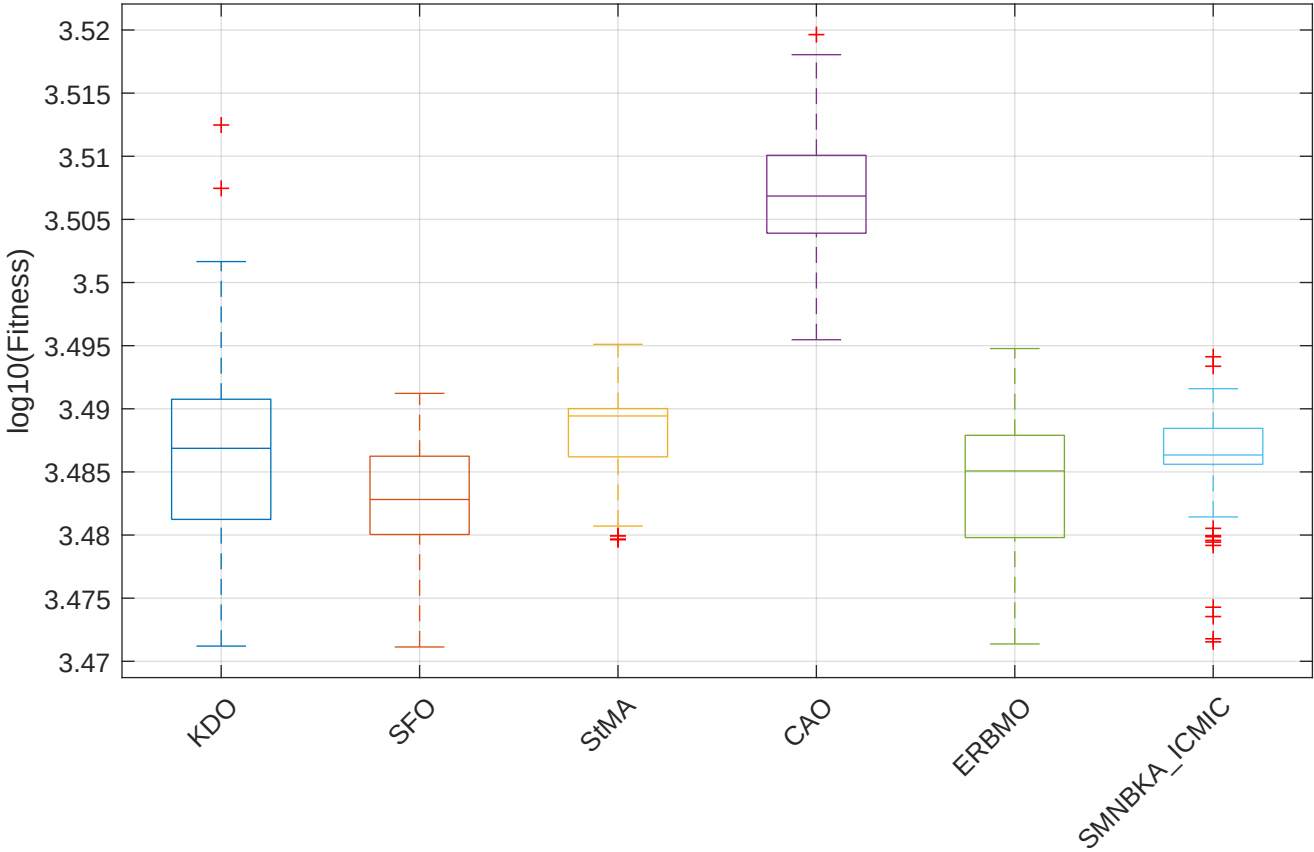
CEC2017 F25 (Numerical) - Boxplot
