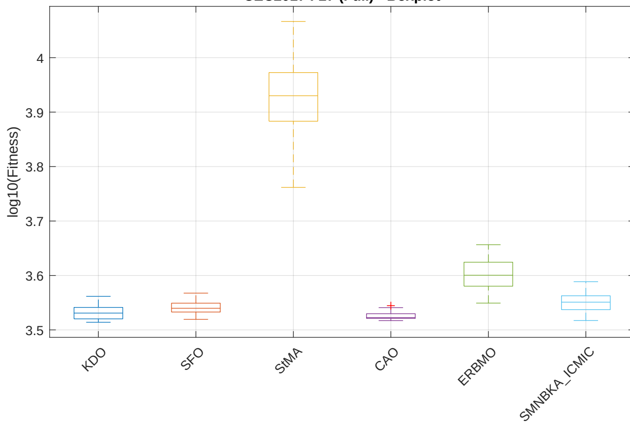
CEC2017 F27 (Full) - Boxplot
