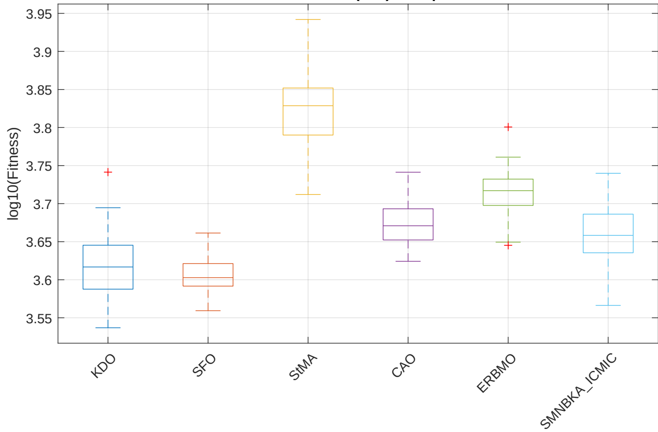
CEC2017 F29 (Full) - Boxplot
