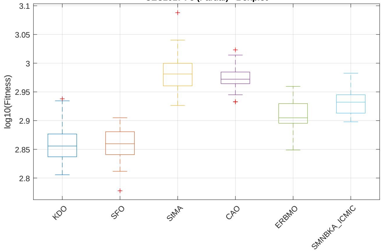
CEC2017 F5 (Partial) - Boxplot
